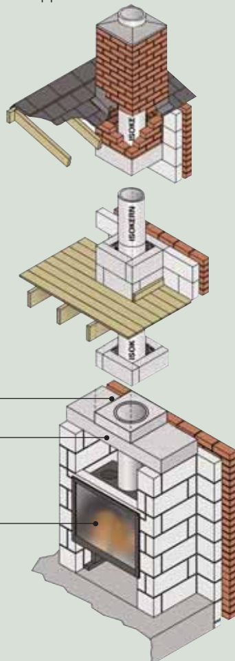
Support block and adaptor for connection to flue pipe
