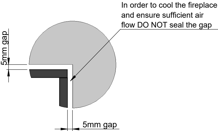
DETAIL Z SCALE 1 : 2
