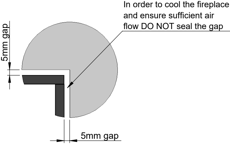
DETAIL Z SCALE 1 : 2
